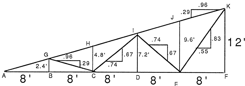
Figure 2.11 Typical loading on roof truss.
