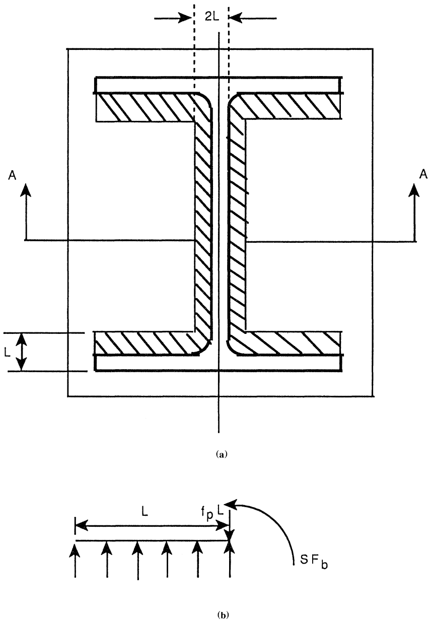
Figure 8.4 Stress action pattern on a baseplate.
