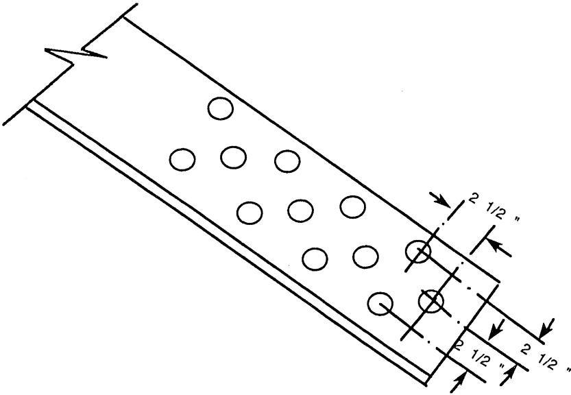
Figure 2.18 Diagonal tension member in the truss system.
