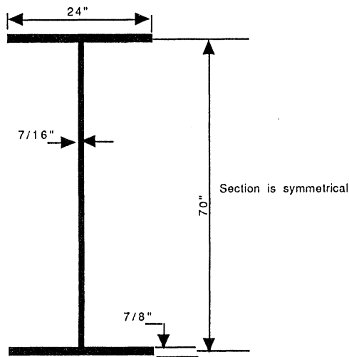
Figure 9.3 Plate girder section.
