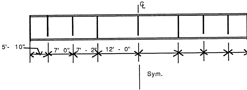
Figure 9.4 Stiffener spacing for plate girder.
