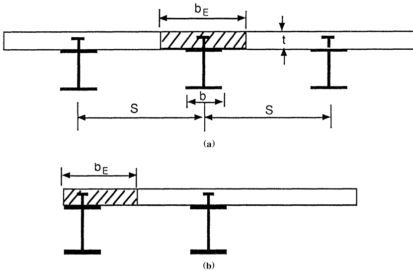
Figure 10.2 Section showing composite construction.
