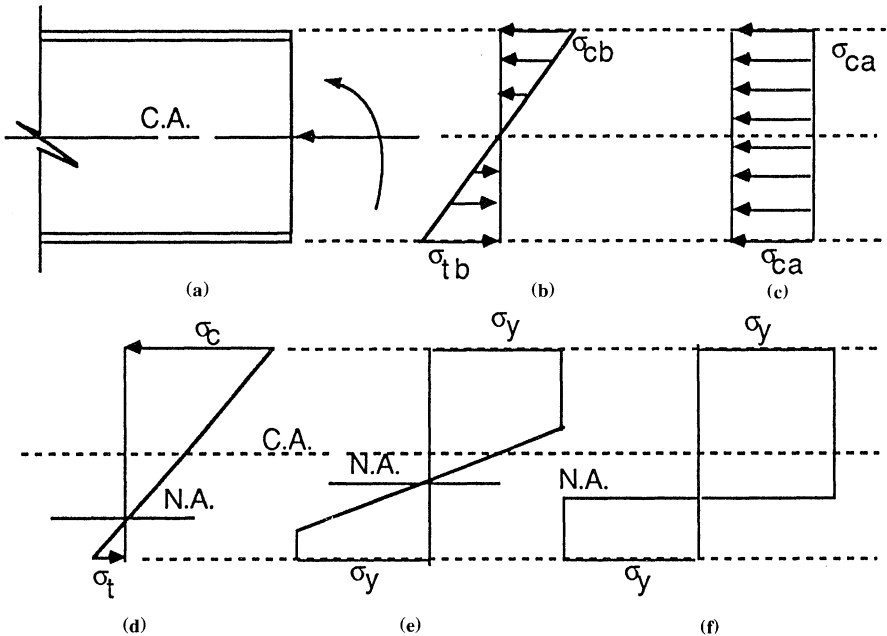
Figure 12.1 Neutral axis falling in the web for combined axial force and bending on beams in the plastic range.
