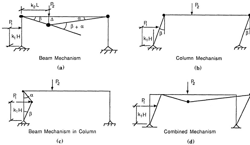
Figure 11.26 Failure mechanism of the portal frame. (a) Beam mechanism. (b) Column mechanism. (c) Beam mechanism in column. (d) Combined mechanism.
