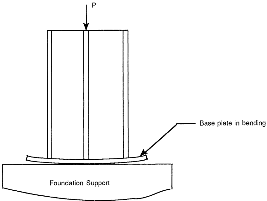
Figure 8.3 Baseplate foundation interaction.
