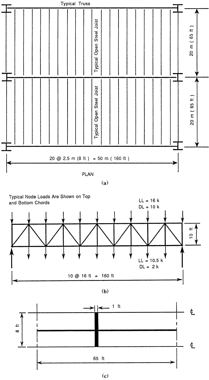
Figure 2.16 (a) Roof plan for a sports arena. (b) Typical node loads on top and bottom chords. (c) Tributary area per foot length of a typical interior truss.
