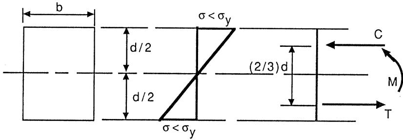
Figure 11.2 Stress distribution diagram: Elastic range.
