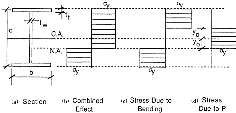
Figure 12.2 Stress distribution due to combined action. (a) Section. (b) Combined effect. (c) Stress due to bending. (d) Stress due to P .
