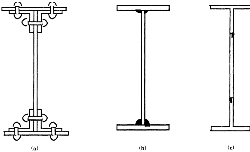
Figure 9.1 Typical plate girder construction.
