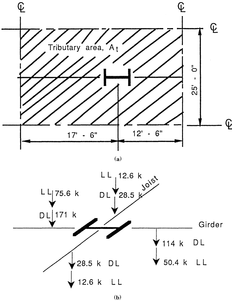
Figure 3.20 Exterior column load calculations. (a) Typical interior column adjacent to exterior bay. (b) Loads on a typical interior column.
