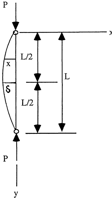
Figure 3.1 Critical axial column load.
