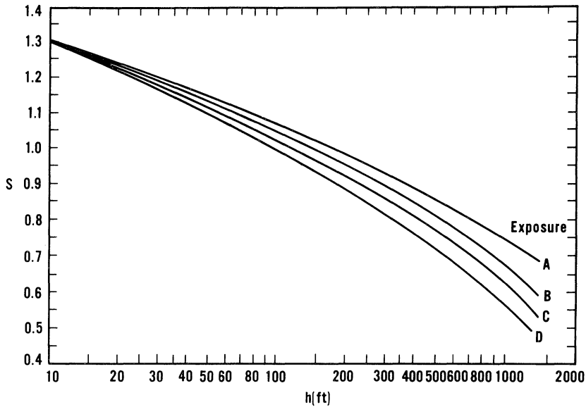
Figure 6.5 Structure size factor S . (Fig. C8 from Minimum Design Loads for Buildings and Other Structures, 1990 by American Society of Civil Engineers.)
