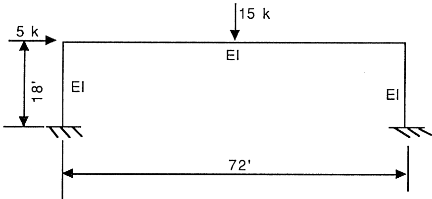
Figure 13.8 Portal frame rigid connection design example.
