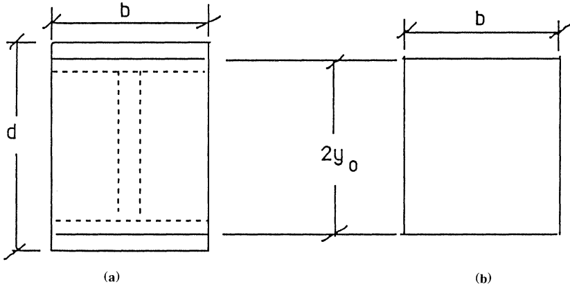
Figure 12.5 Generalized section.
