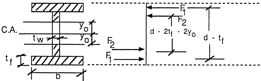
Figure 12.3 Determination of position of the neutral axis in the web.
