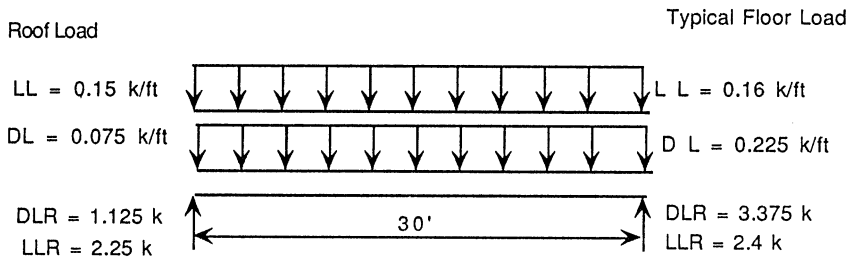
Figure 3.9 Loads on a typical roof or floor joist.
