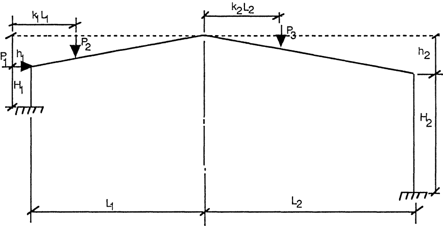
Figure 11.28 Gable frame.
