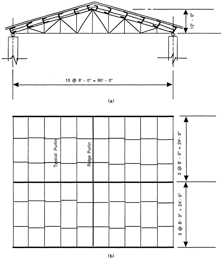
Figure 2.10 Long-span roof truss system. (a) Typical roof truss. (b) Plan of roof framing system.
