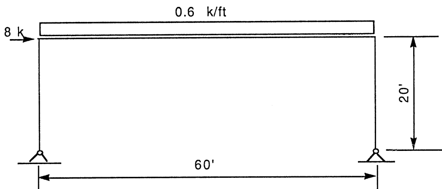
Figure 13.4 Portal frame example.
