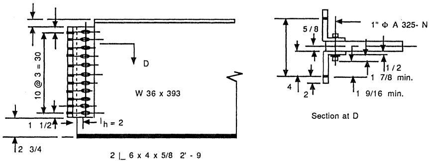
Figure 7.8 Standard column-girder connection.
