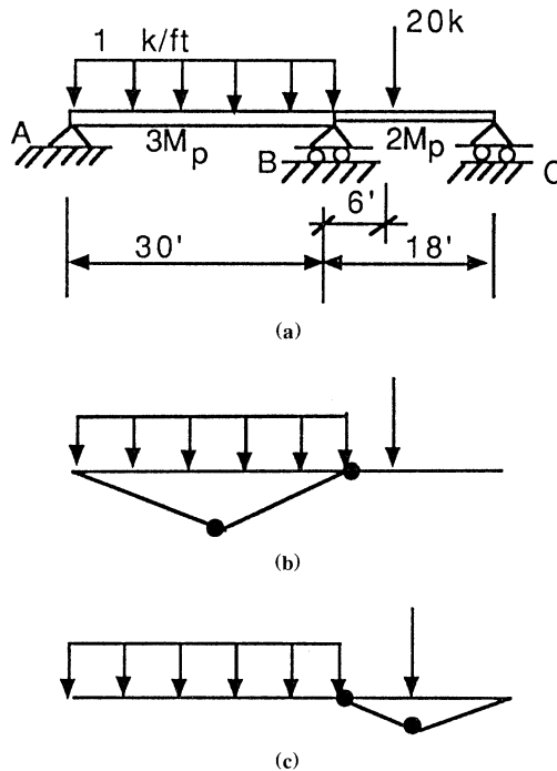
Figure 11.20 Failure mechanism of a continuous beam, two spans.
