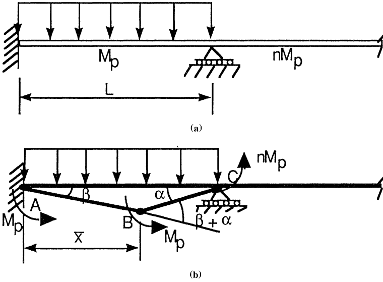
Figure 11.18 Continuous beam at one end and fixed at the other with variable sections and a uniformly distributed load.
