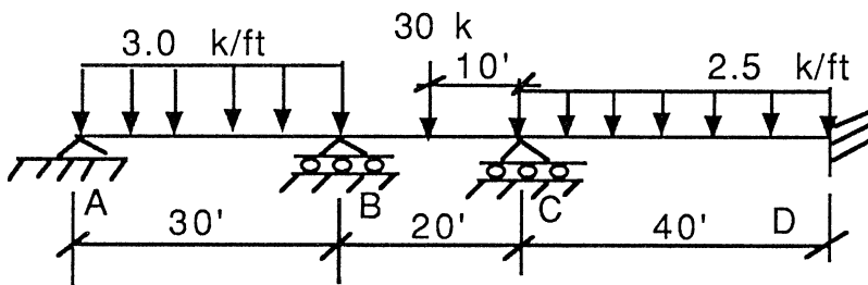
Figure 11.23 Three-span continuous beam.
