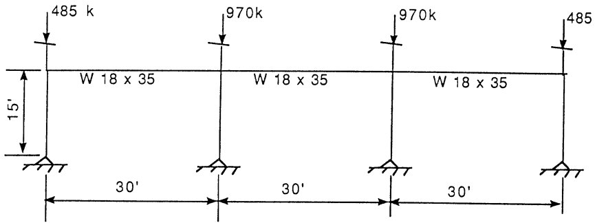
Figure 3.16 Unbraced frame of a multistory building.
