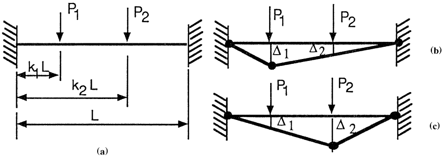
Figure 11.17 Fixed end beam with two concentrated loads.
