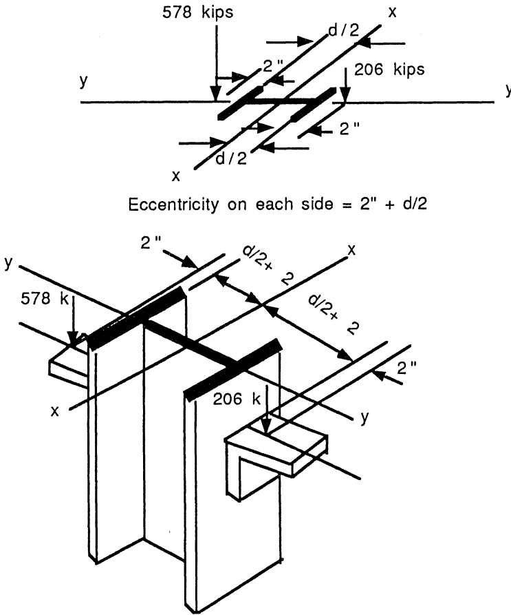
Figure 3.22 Determination of eccentricity of a typical column beam connection.
