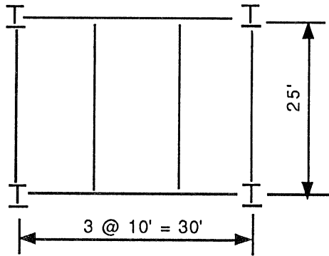
Figure 10.13 Typical floor bay.
