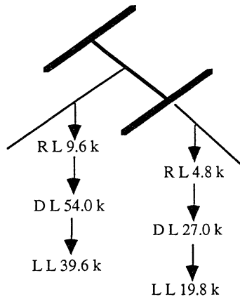
Figure 3.21 Corner column load calculations.
