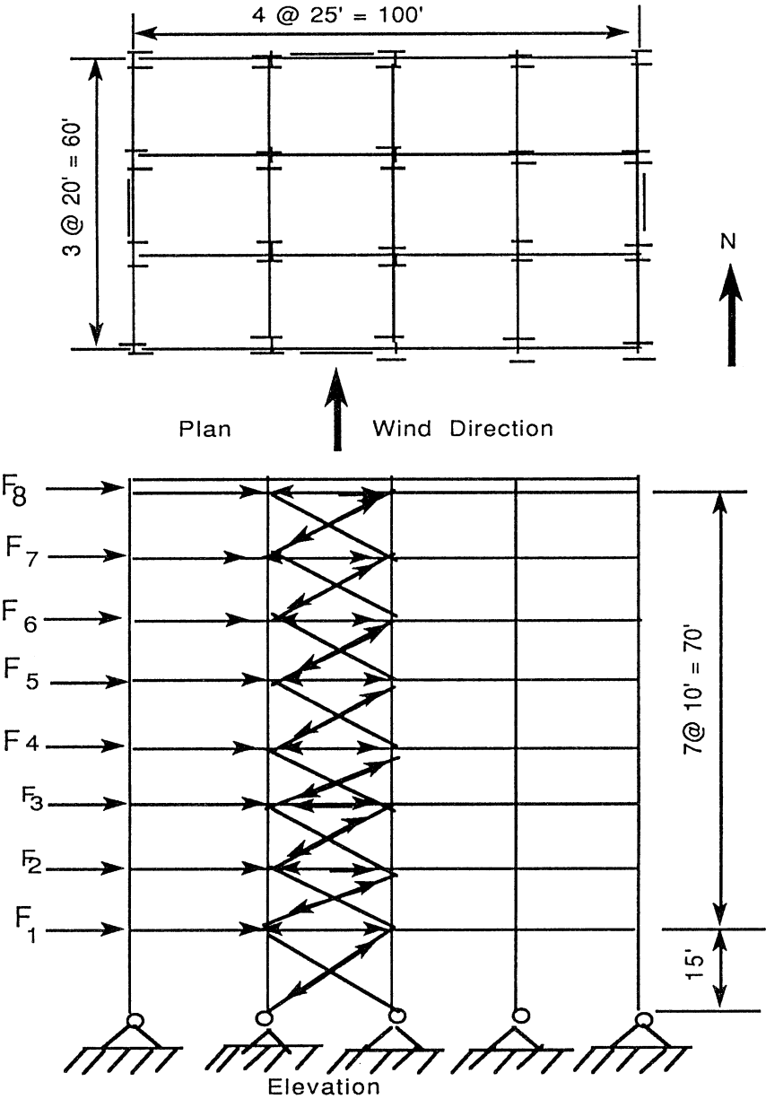
Figure 6.7 Transfer of wind forces into the building frame system of braced frames with standard bolt connections.
