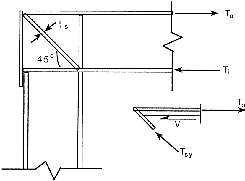
Figure 13.5 Stiffener design for corner connections.
