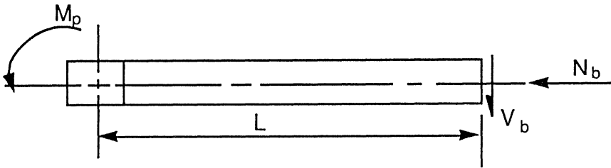
Figure 13.3 Free-body diagram of one leg of a straight corner connection.
