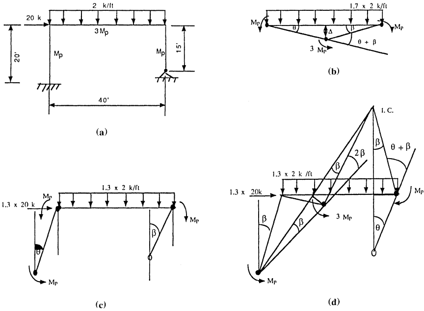
Figure 12.6 Portal frame design example.
