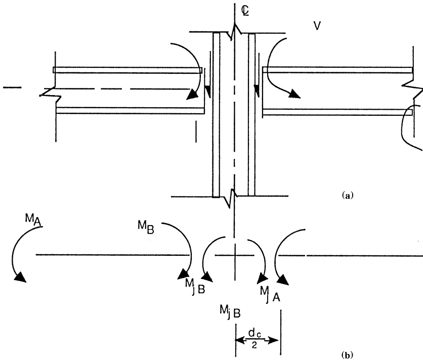
Figure 14.3 Girder-column moment and shear design.
