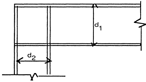
Figure 13.10 Straight corner.
