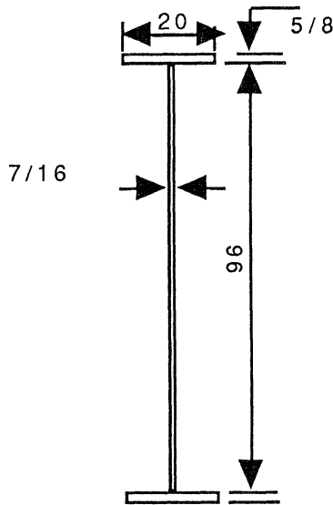
Figure 9.7 Plate girder section.
