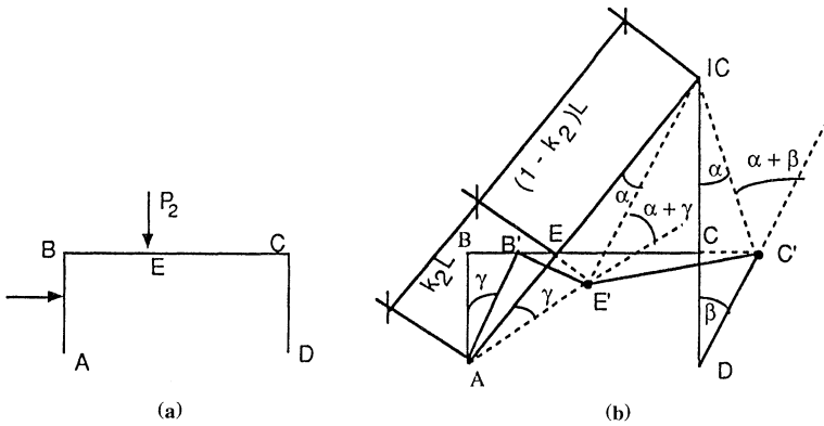
Figure 11.27 Kinematics of the portal frame.
