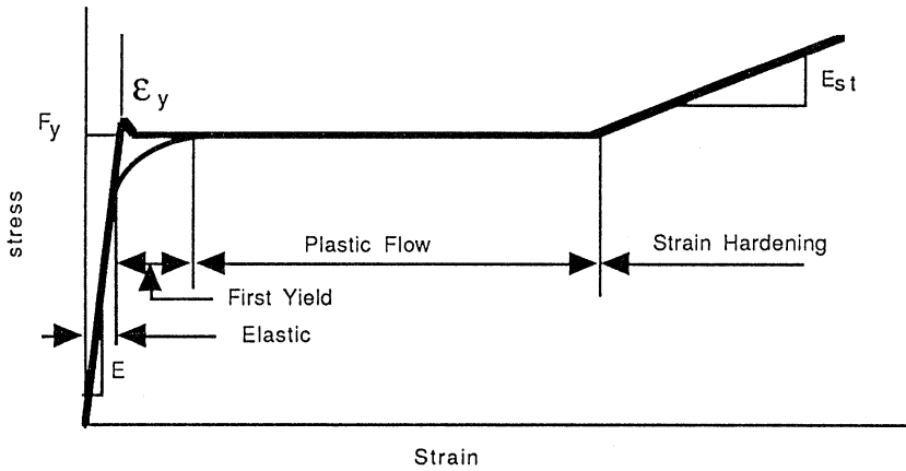
Figure 2.3 Stress vs. strain for structural steel.
