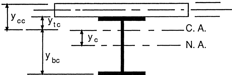
Figure 10.5 Centroidal axis of composite section.
