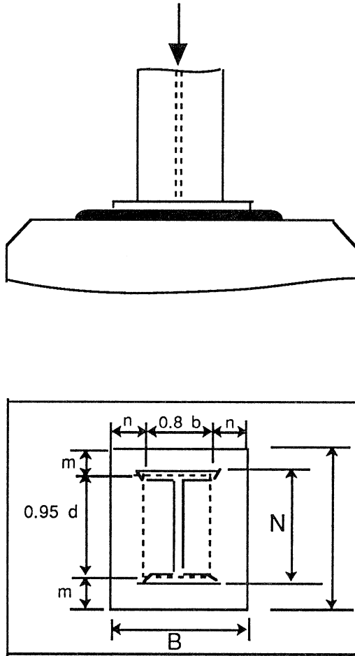
Figure 8.2 Column baseplate: AISC procedure.
