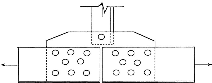
Figure 2.15 Lower chord connection.
