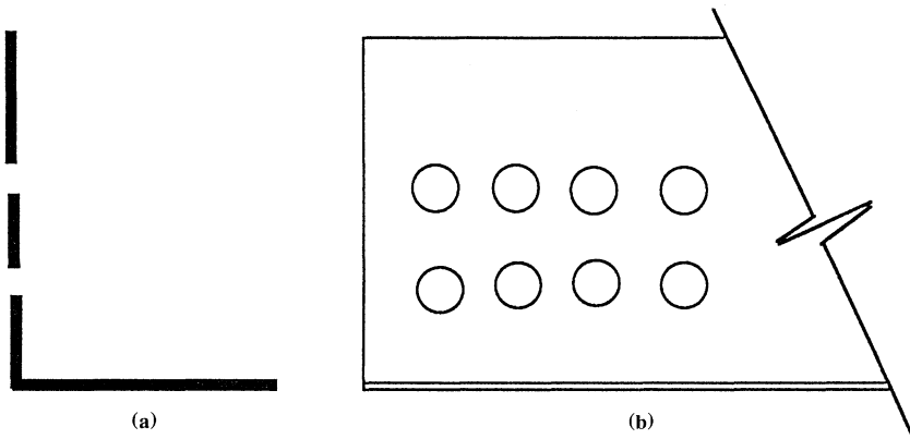
Figure 2.5 Multiple-bolt connection. (a) Cross section. (b) Side view.
