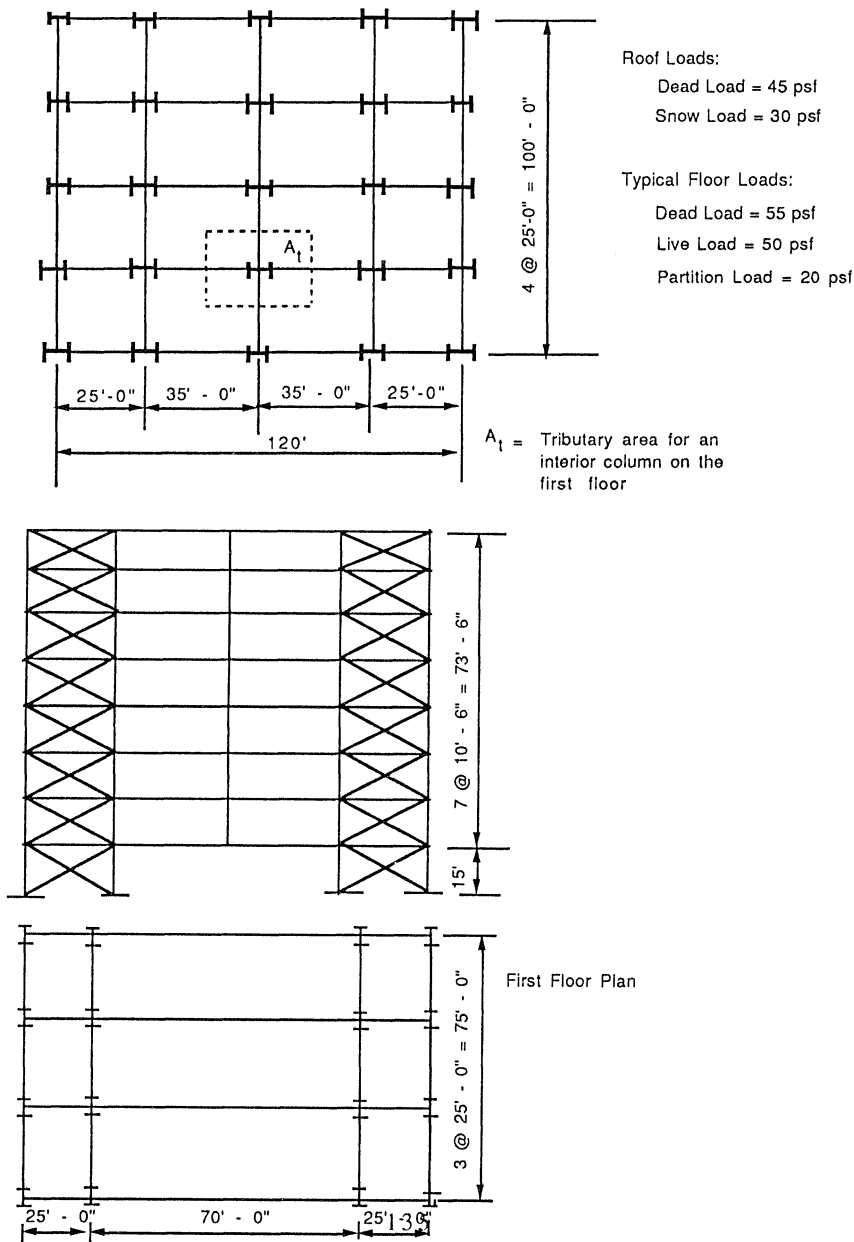
Figure 3.17 Floor and elevation of a seven-story building.
