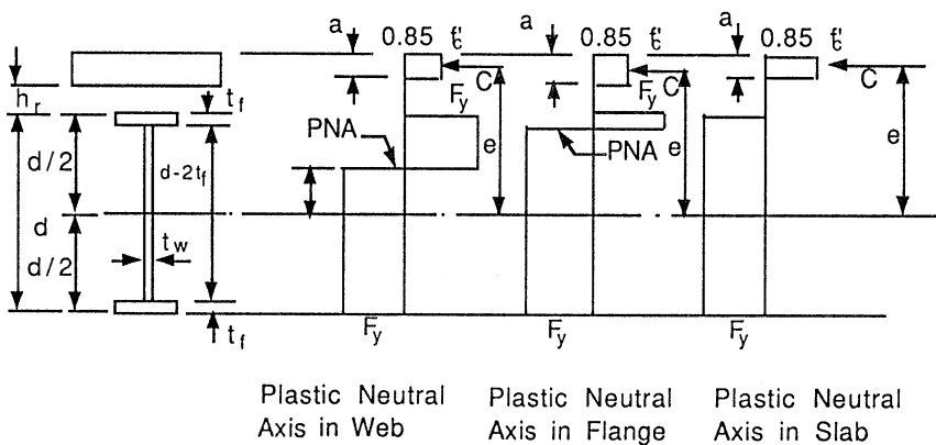
Figure 10.10 Use of plastic stress method in composite beams.
