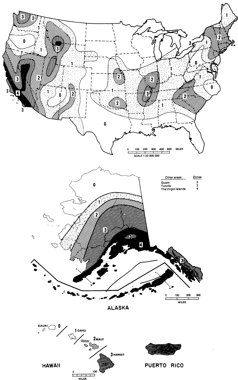
Figure 6.12 Seismic zone chart for the United States and its territories. (Courtesy of American Society of Civil Engineers, Minimum Design Loads for Buildings and Other Structures.)
