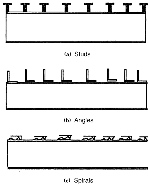
Figure 10.1 Types of shear connectors. (a) Studs. (b) Angles. (c) Spirals.
