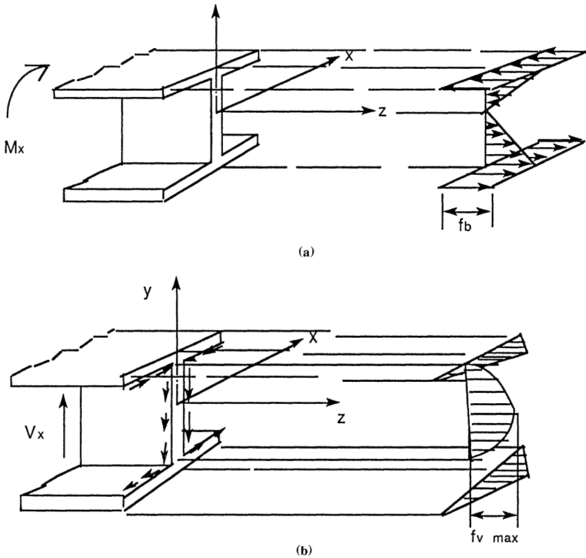
Figure 4.3 (a) Normal bending stress. (b) Shear bending stress.
