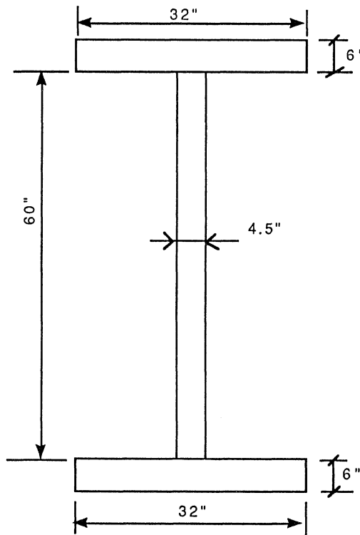
Figure 9.11 Trial dimensions for the plate girder.
