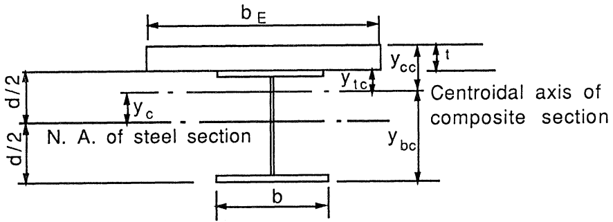
Figure 10.7 Location of neutral axis of a composite section.
