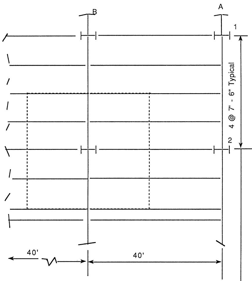
Figure 3.11 Typical interior column tributary area.
