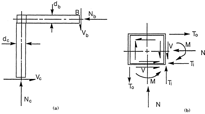
Figure 13.2 Free-body diagram of corner connection.
