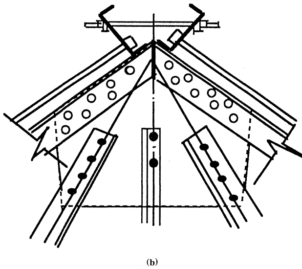
Figure 2.9 Roof purlin and tie-rod system. (a) Plan of roof frame. (b) Sag rods for roof purlins.
