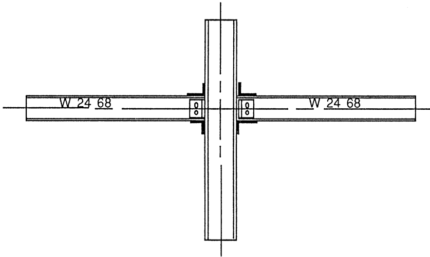
Figure 3.19 Interior column-girder connection.
