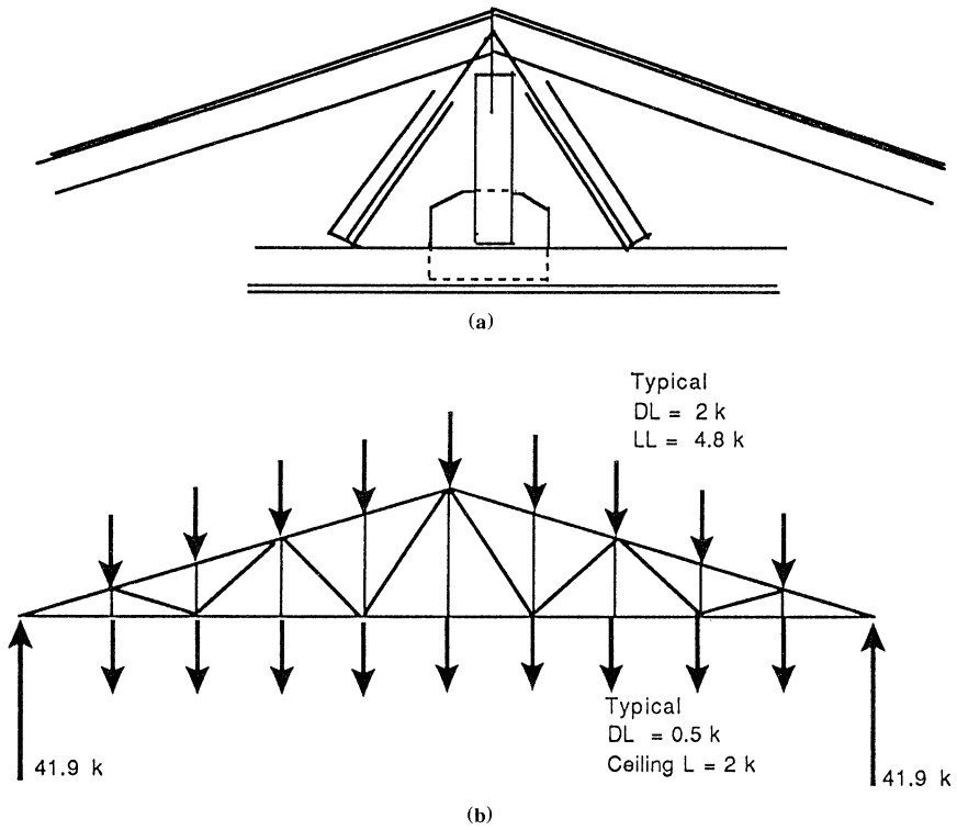
Figure 2.12 Member direction cosines for truss system. (a) Truss connection. (b) Truss loading.
