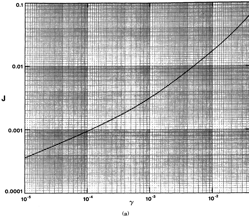
Figure 6.6a Pressure profile factor. (Fig. C6 from Minimum Design Loads for Buildings and Other Structures, 1990 by American Society of Civil Engineers.)
