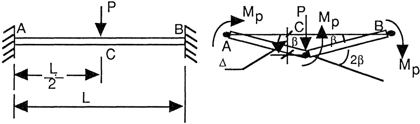
Figure 11.13 Fixed end beam with a concentrated load at midspan.
