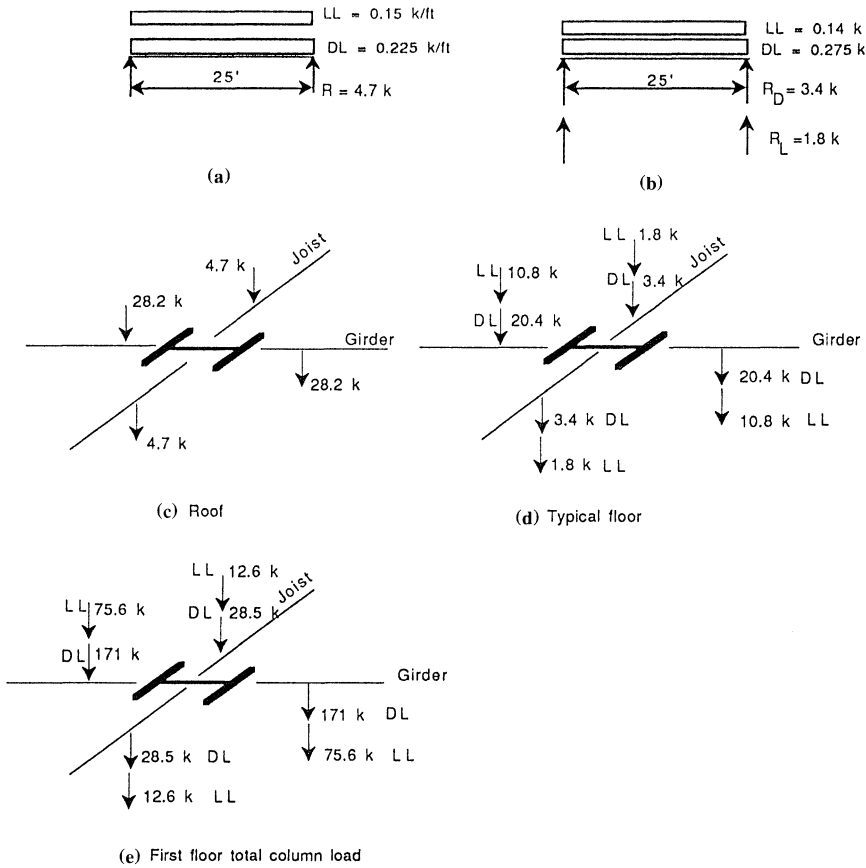
Figure 3.18 Interior column load calculations for the first floor. (a) Typical roof joist loads. (b) Typical floor joist loads. (c). Roof. (d) Typical floor. (e) First floor total column load.
