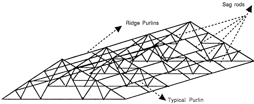
Figure 2.8 Roof truss framing system.
