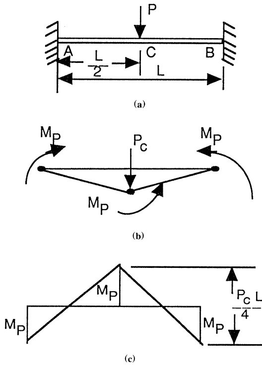
Figure 11.14 Failure mechanism of a fixed end beam with a concentrated load at midspan.
