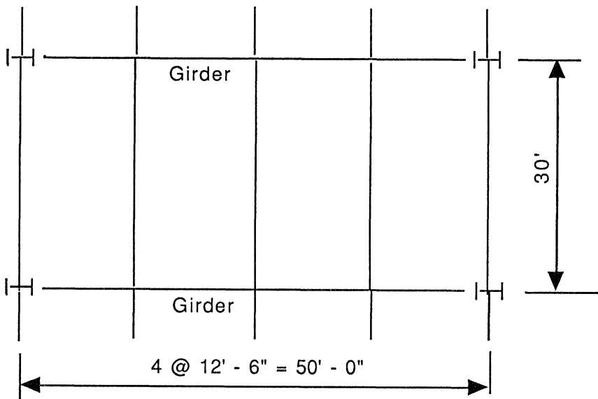
Figure 7.11 Typical floor framing system.
