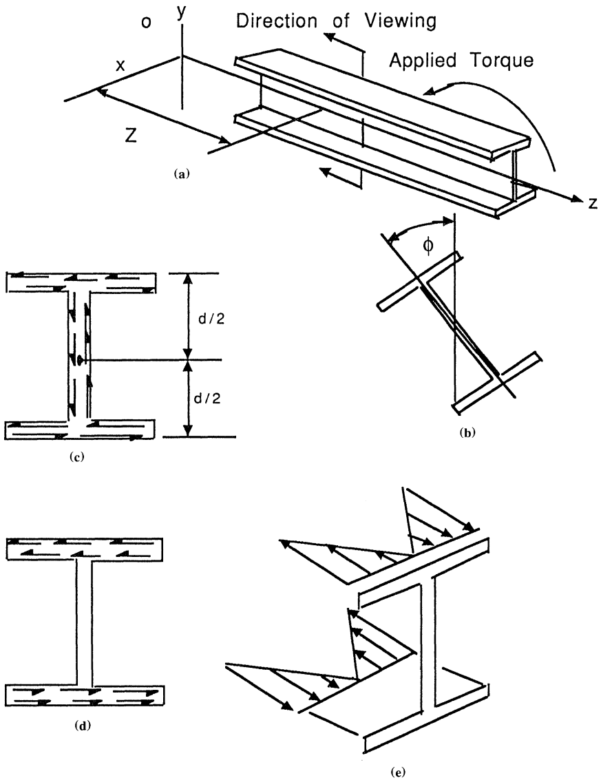
Figure 5.2 Torsional stresses and stress orientation. (a) General orientation of beam. (b) Positive angle of rotation. (c) Pure torsional shear. (d) Warping shear stresses. (e) Warping normal stresses.
