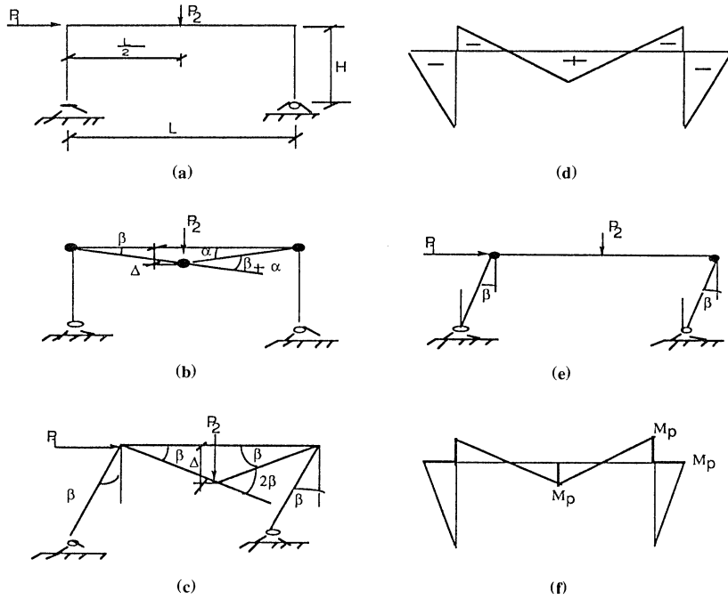
Figure 11.24 Portal frame.
