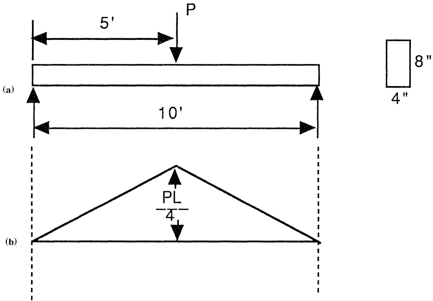
Figure 11.11 Simply supported beam with a concentrated load at midspan.
