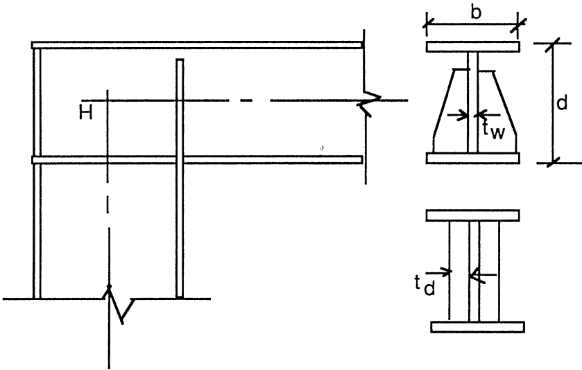
Figure 13.9 Design of stiffeners for rigid connections.
