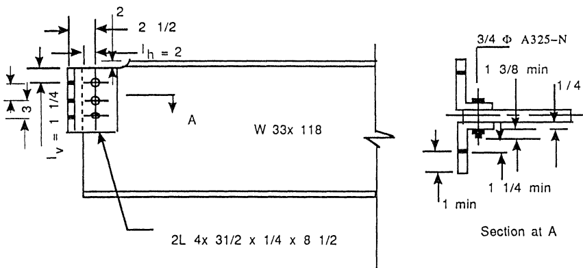
Figure 7.4 Typical beam-to-column connection.
