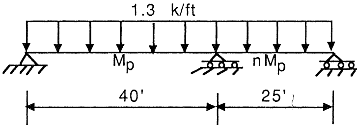
Figure 11.22 Two-span continuous beam with a variable section and uniformly distributed load.
