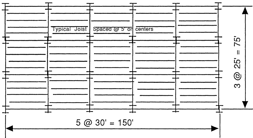
Figure 3.6 Seven-story building.
