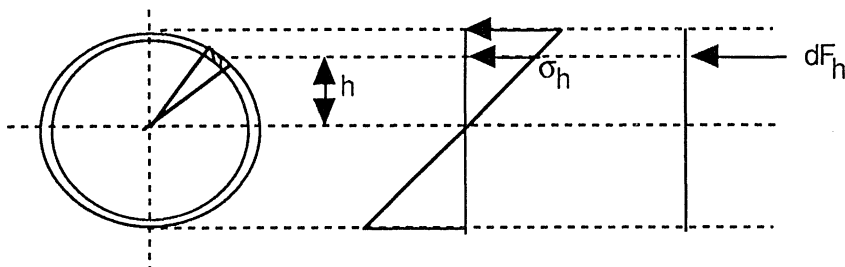
Figure 11.7 Hollow tube section.
