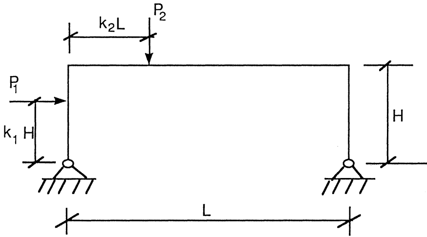
Figure 11.25 Portal frame with concentrated loads at any point on column and girder.
