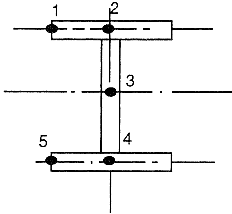
Figure 5.8 Stress location designation for beams in torsion.
