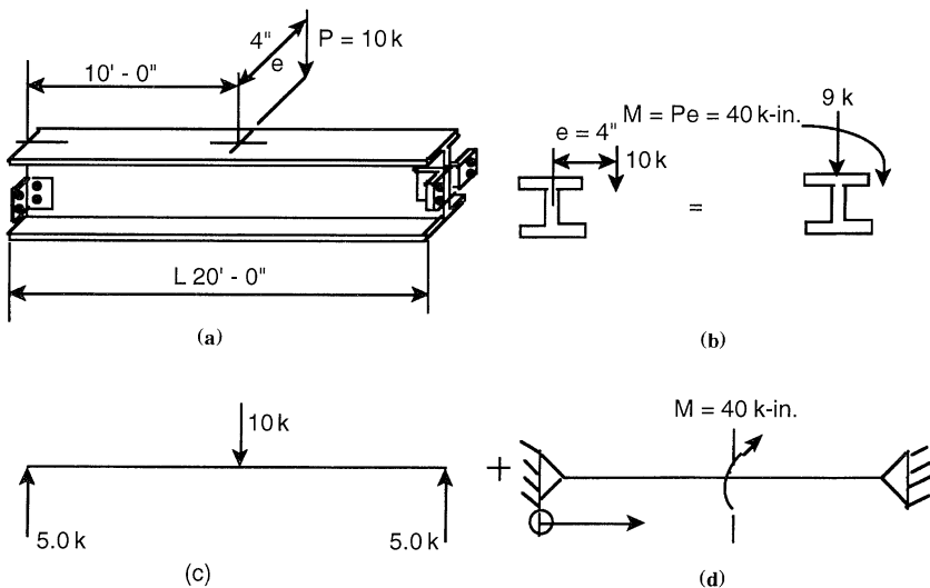
Figure 5.7 Simply supported beam in torsion.
