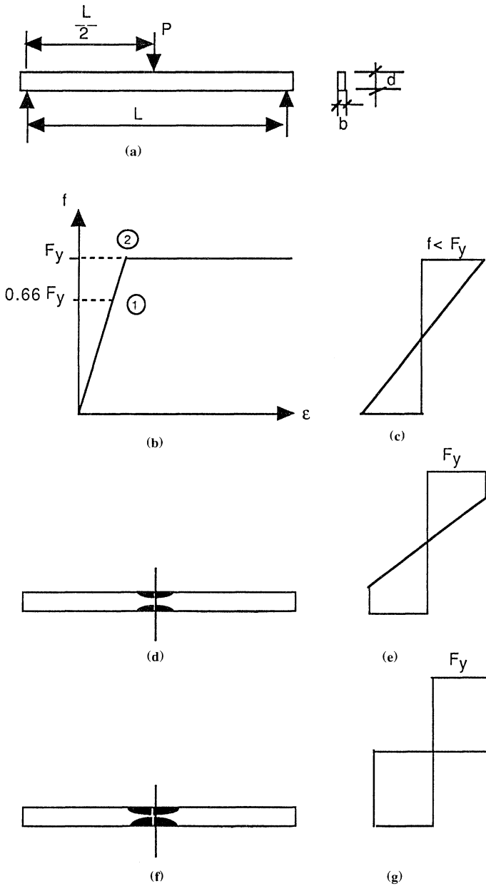
Figure 11.10 Development of the plastic hinge.
