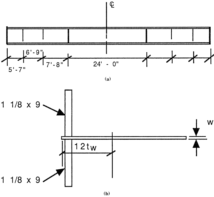
Figure 9.8 End bearing stiffener. (a) Modified dimensions. (b) Stiffener spacing.
