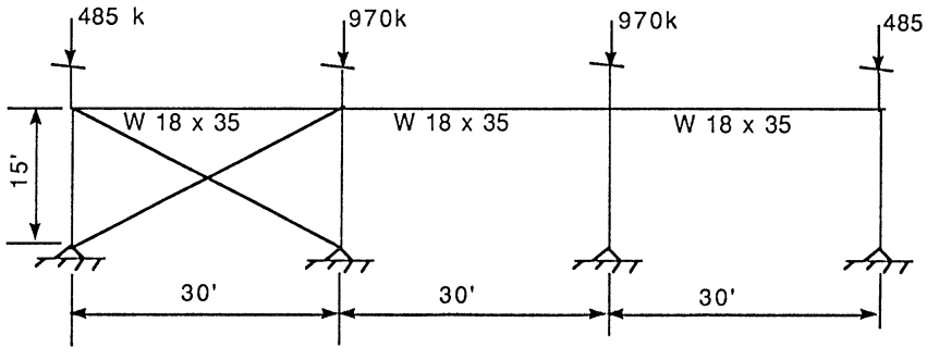
Figure 3.15 Braced frame of a multistory building.
