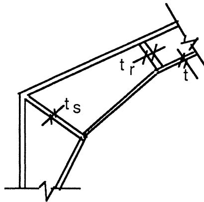
Figure 13.13 Haunched corner rigid connection proportions.
