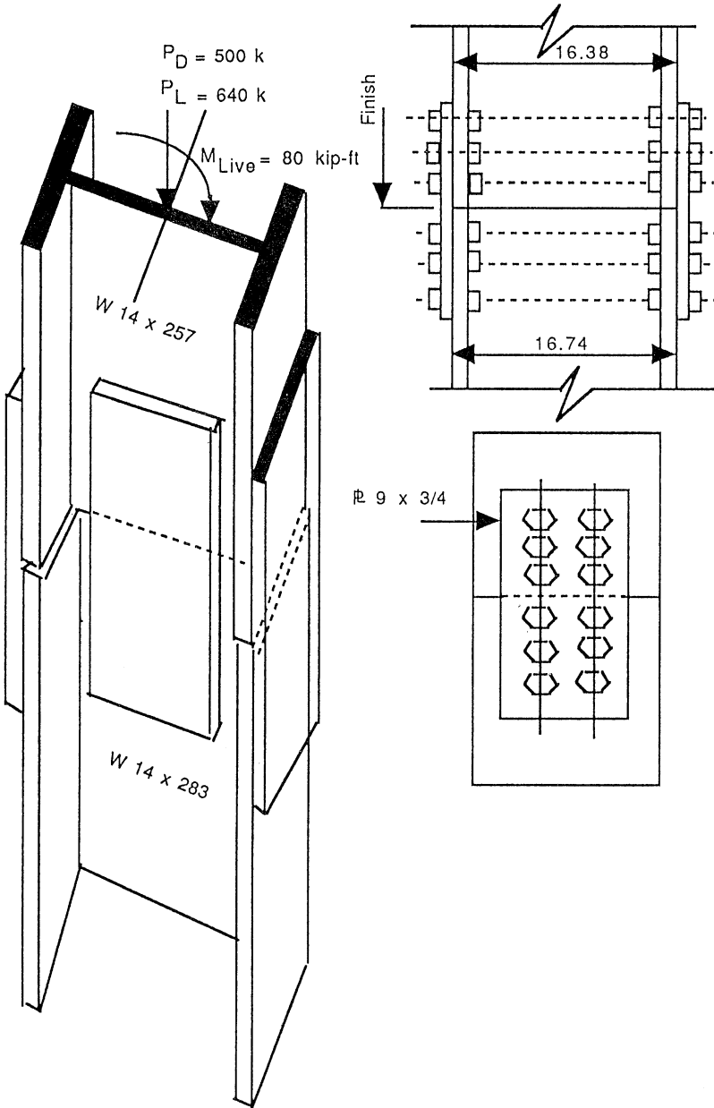
Figure 7.1 Column splice.
