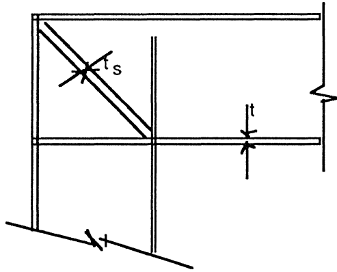
Figure 13.11 Stiffener for a straight corner.
