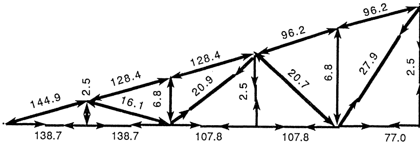
Figure 2.14 Member forces in the truss system.
