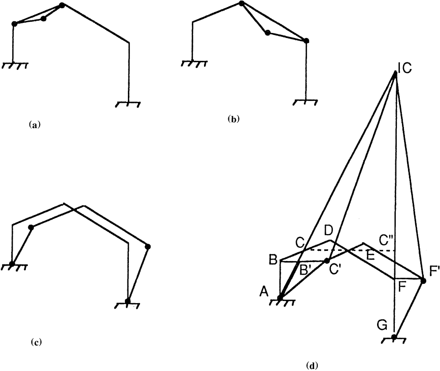
Figure 11.29 Kinematics of the gable frame.
