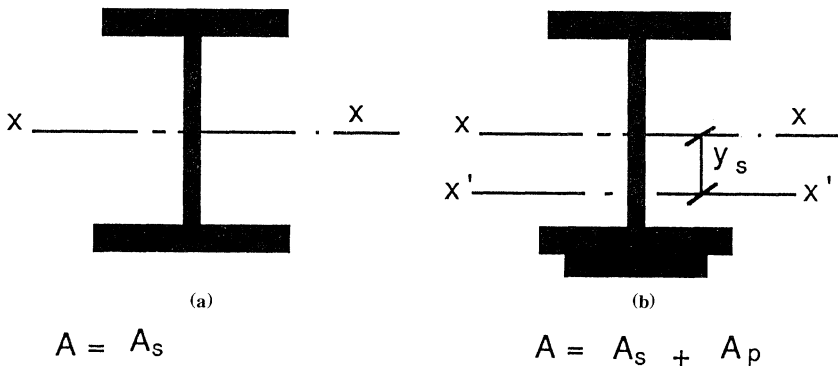
Figure 10.3 Cover plates.
