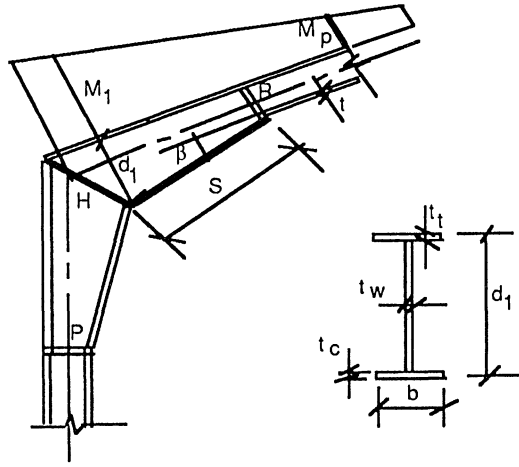
Figure 13.12 Haunched corner rigid connection for a gabled frame.
