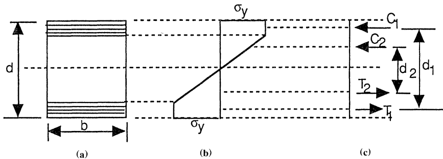
Figure 11.4 Stress distribution: Plastic-elastic range.
