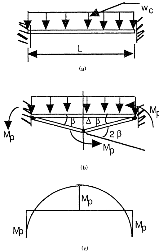
Figure 11.15 Failure mechanism of a fixed end beam with a uniformly distributed load.
