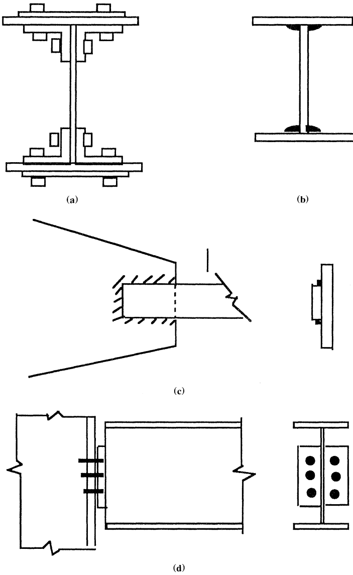
Figure 7.2 Standard column connections.
