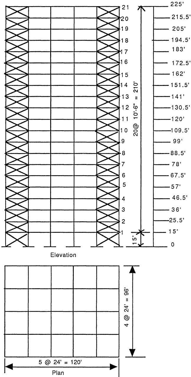
Figure 6.11 Twenty-one-story building frame system.
