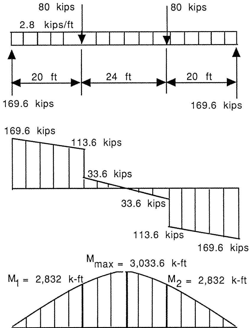
Figure 9.2 Plate girder loading, shear, and bending moment diagrams.
