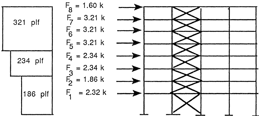
Figure 6.8 Wind shear against building floors.
