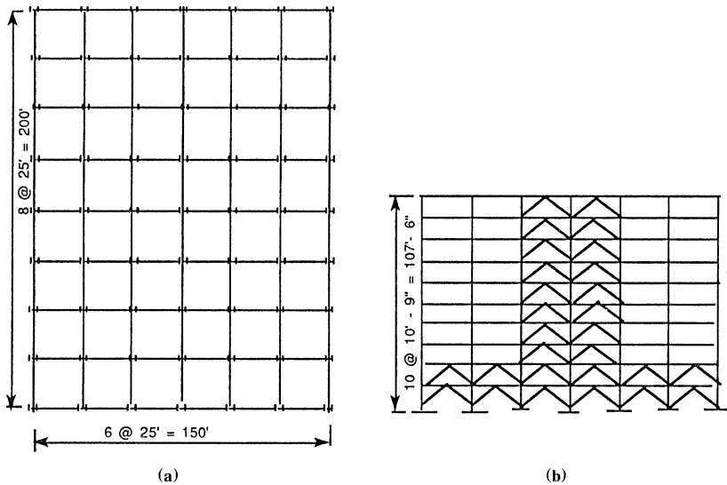
Figure 6.13 Ten-story building for seismic design. (a) Plan. (b) Elevation N-S.
