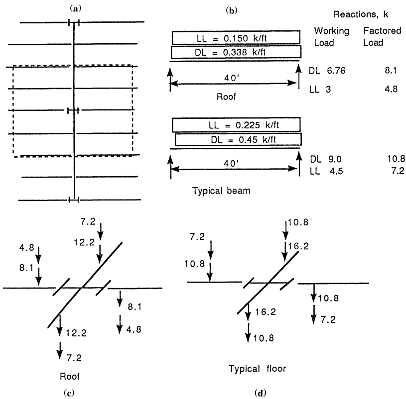
Figure 3.12 Typical load calculation on an interior column.
