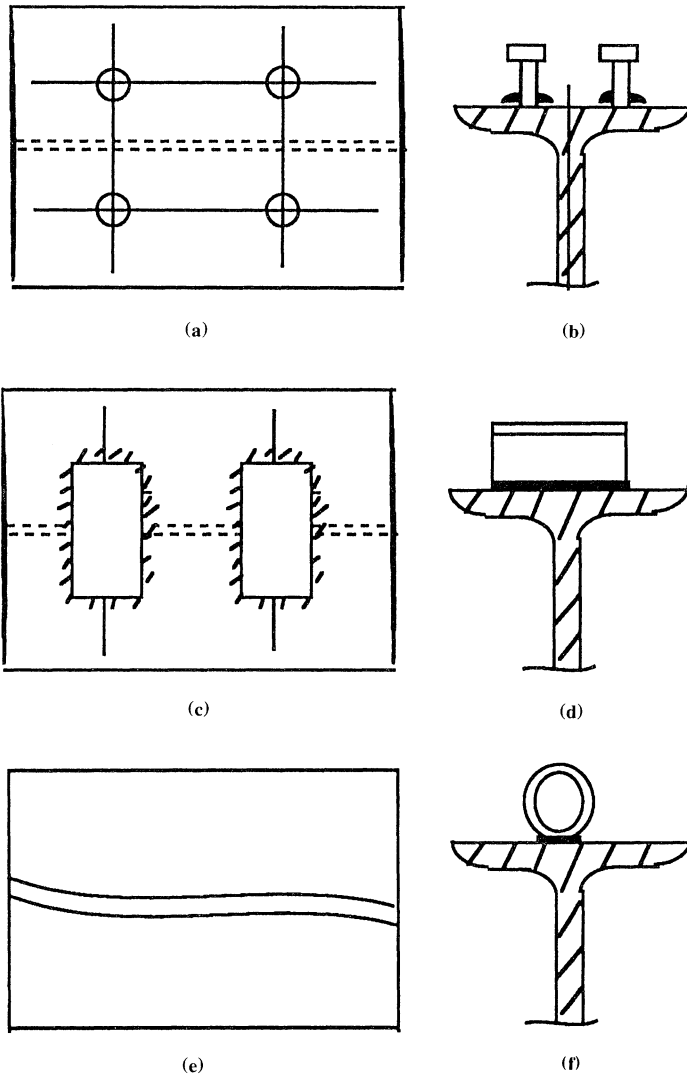
Figure 10.9 Types of shear connectors.
