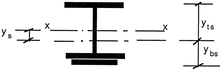
Figure 10.4 Neutral axis of W-flange sections with cover plates.
