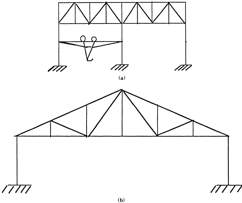
Figure 2.1 Typical structures with tension members.
