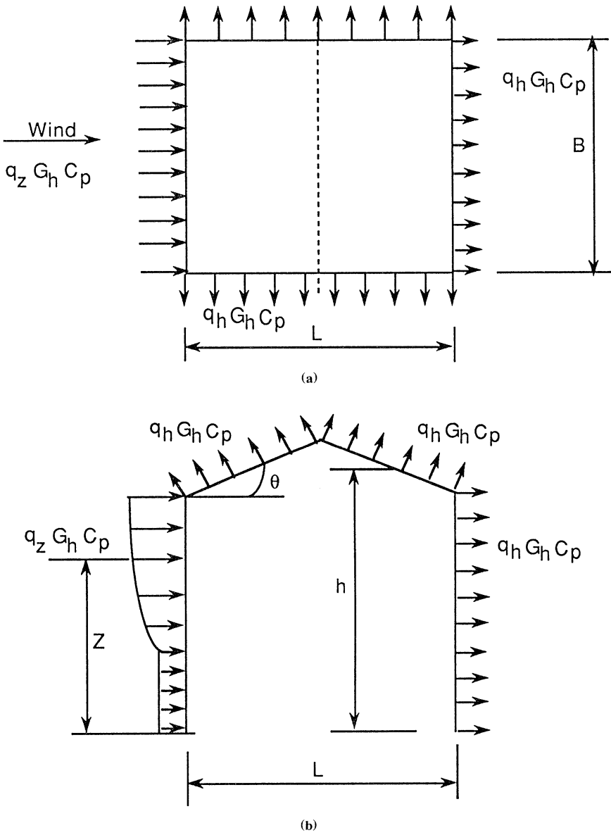
Figure 6.4 Wind drag coefficients for ordinary buildings. (a) Plan. (b) Elevation.
