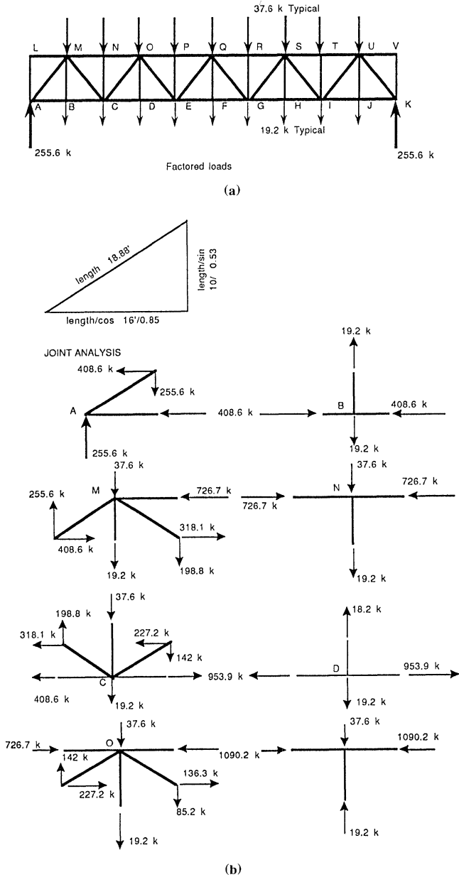
Figure 2.17 (a) Factored load on the truss system. (b) Resolution of member forces for the truss system. (c) Member Forces in the truss.
