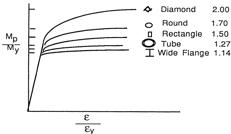
Figure 11.6 Shape factors for various sections.
