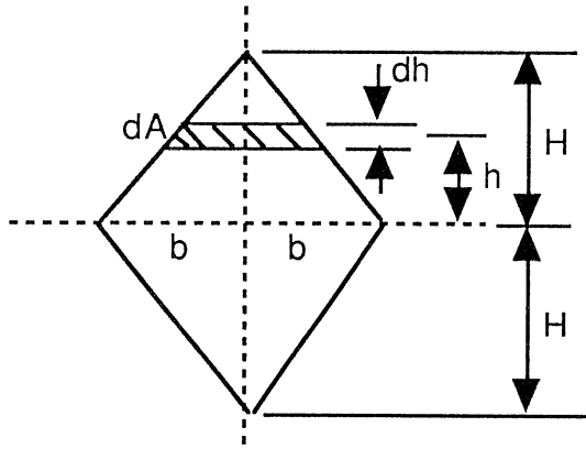
Figure 11.9 Diamond section.
