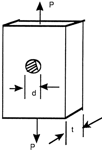
Figure 2.4 Single-bolt connection.
