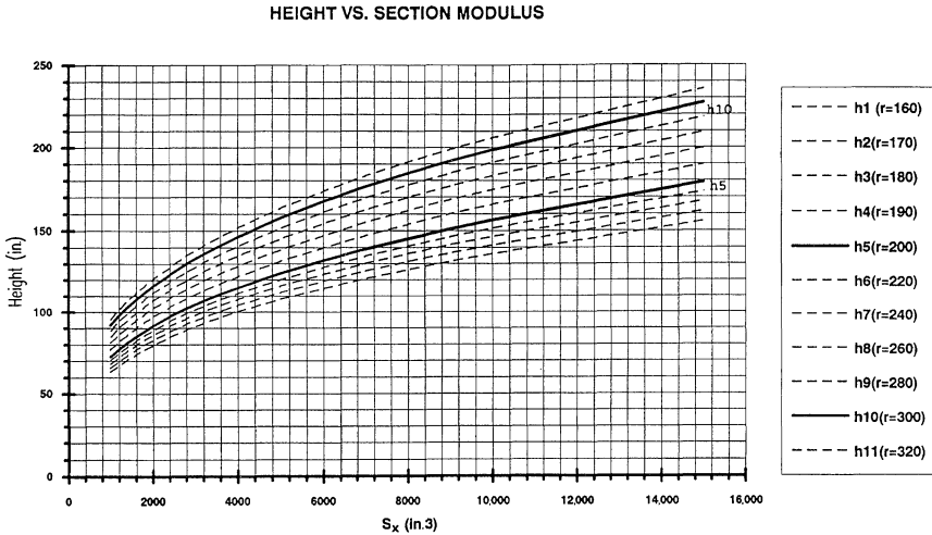
Figure 9.12 Trial height charts for plate girders.
