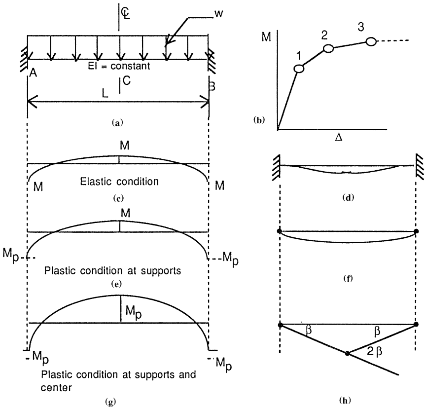
Figure 11.12 Fixed end beam with a uniform load on entire span.
