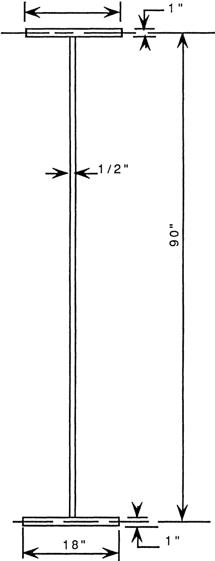
Figure 9.13 Final dimensions for the plate girder.
