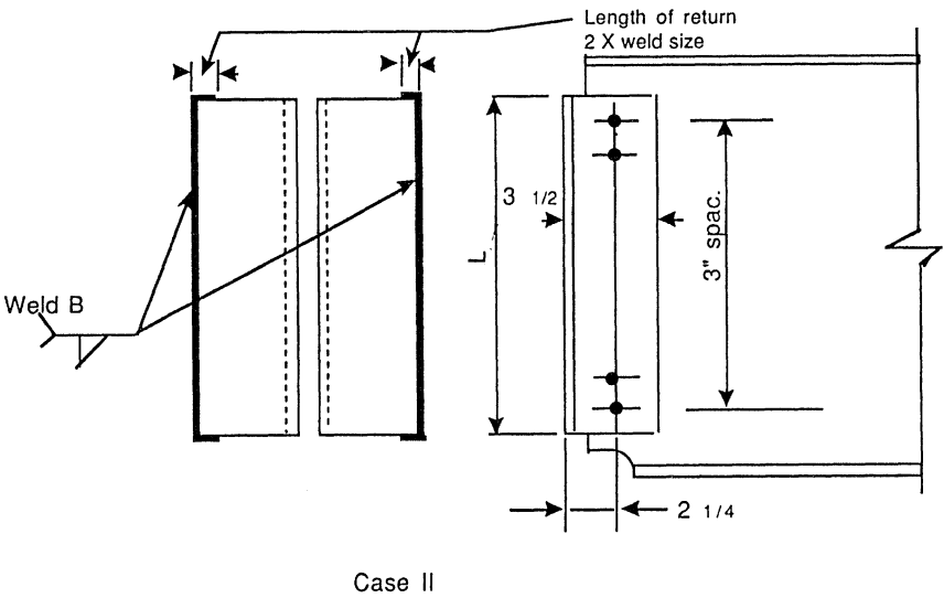
Figure 7.10 Typical welded connection: Case II.
