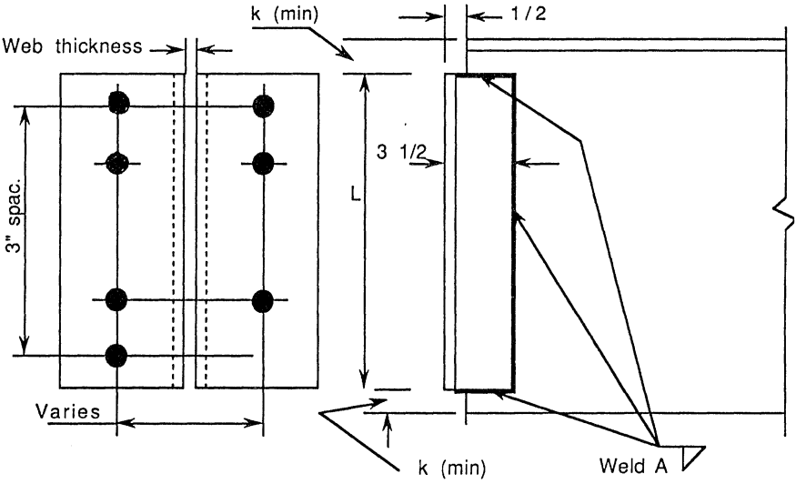
Figure 7.9 Typical welded connection: Case I.
