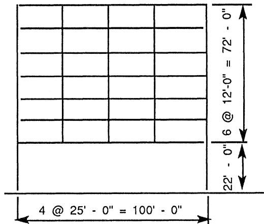
Figure 9.9 Seven-story building with no interior columns on first floor.
