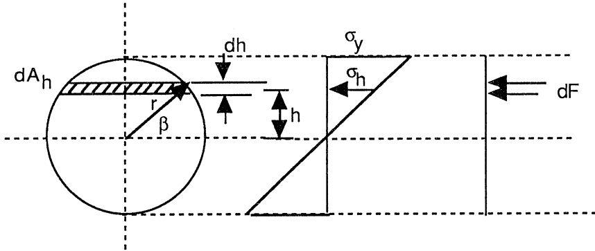
Figure 11.8 Circular section.
