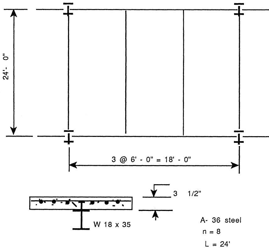
Figure 10.6 Typical floor frame: Interior bay.
