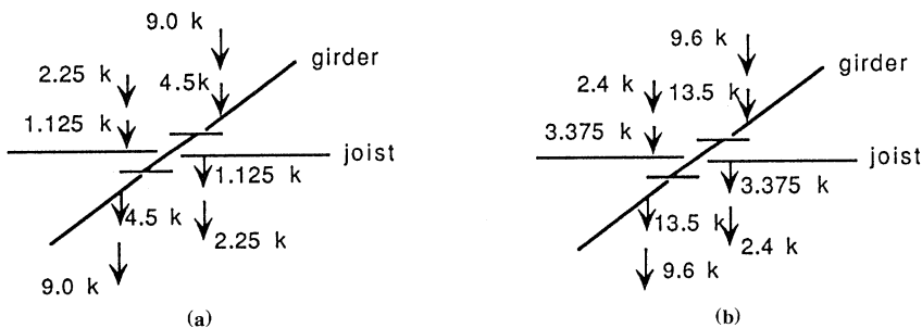
Figure 3.10 Loads on a typical interior column. (a) Roof loads. (b) Floor loads.
