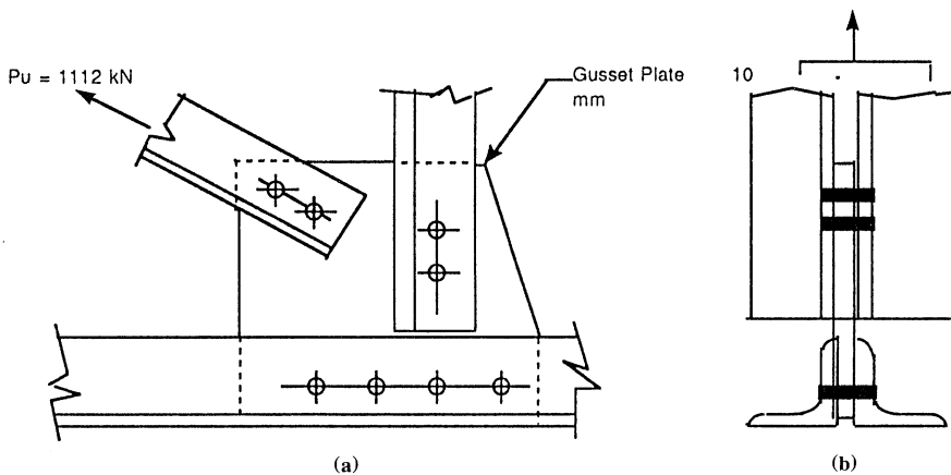
Figure 2.19 Tension member using the SI system of measurement.
