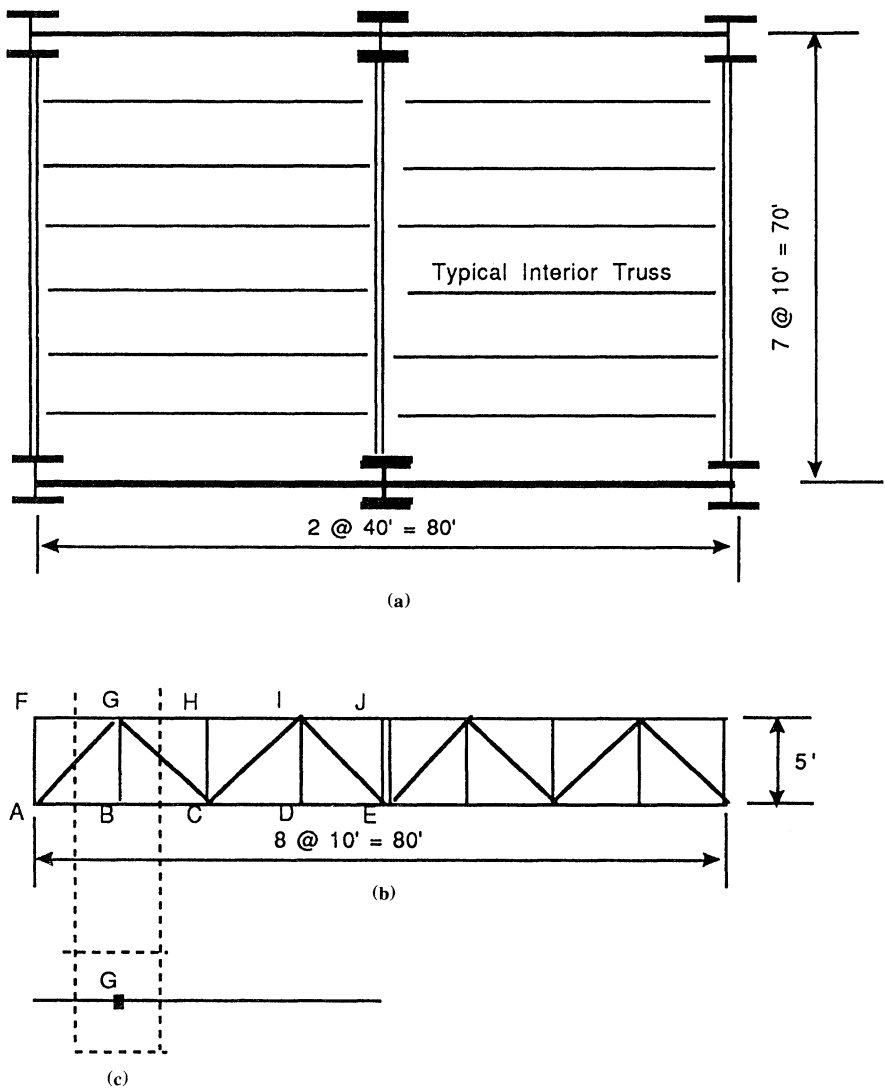
Figure 3.3 Building floor plan.
