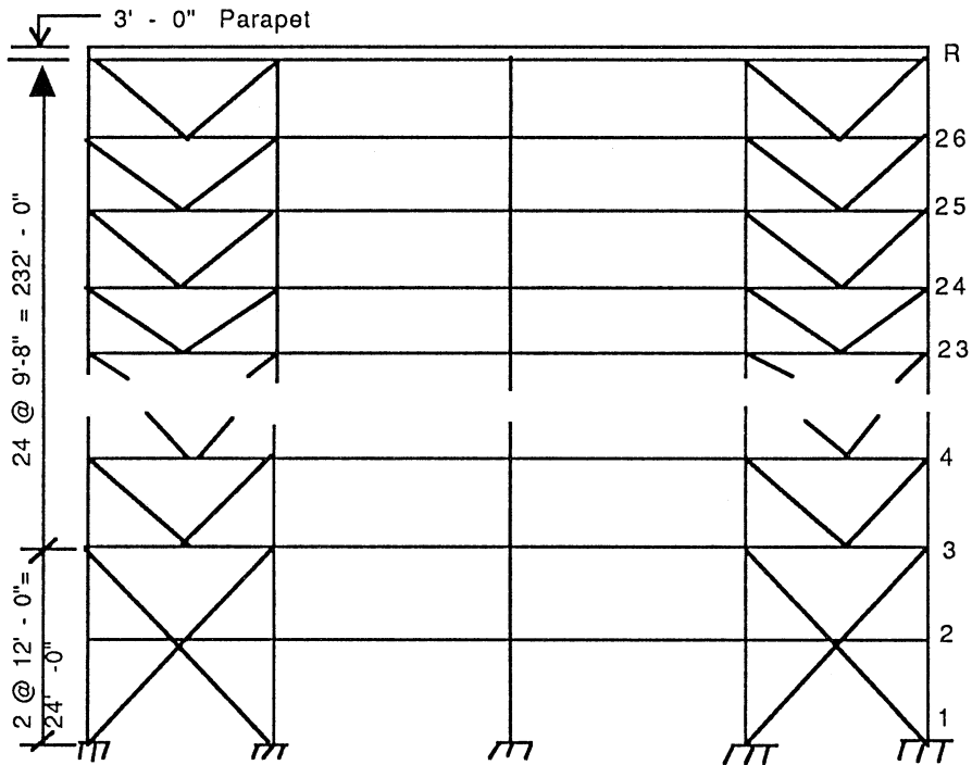
Figure 14.2 Evaluation of 27-story building.
