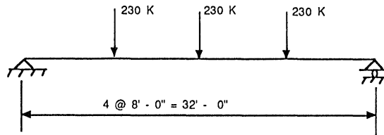
Figure 7.7 Large concentrated loads on a 32-ft girder.
