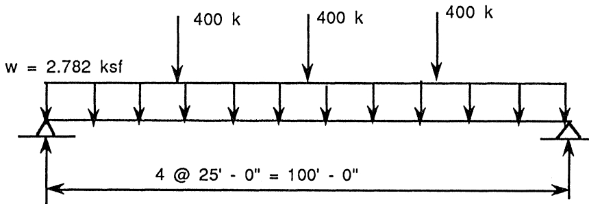
Figure 9.10 Loading on the plate girder for the first floor.
