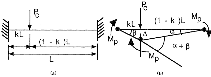
Figure 11.16 Fixed end beam with one single concentrated load at any point.
