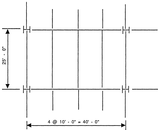
Figure 7.3 Typical interior bay framing system.
