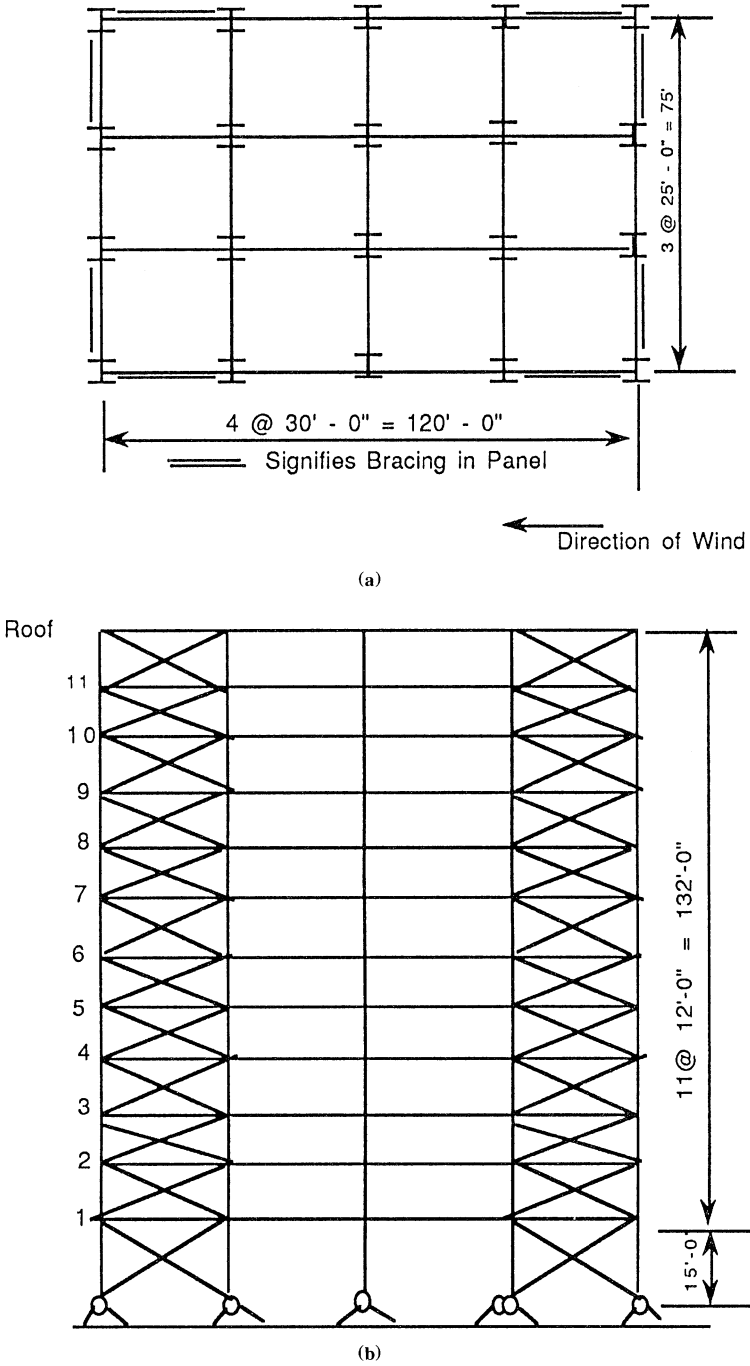
Figure 6.1 Wind against a multistory building. (a) Plan. (b) Elevation.
