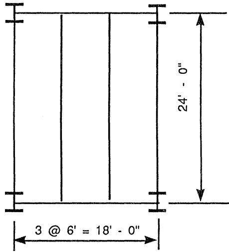
Figure 10.8 Floor frame: Typical Bay.
