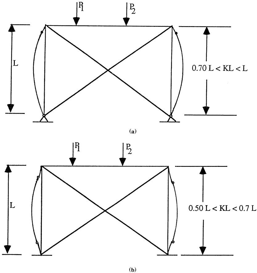
Figure 3.13 Braced frames. (a) Hinged support. (b) Fixed support.
