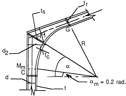
Figure 13.14 Curved haunched rigid connection.
