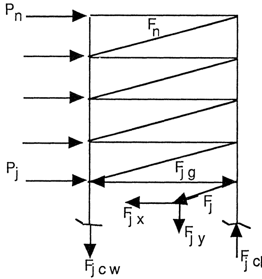
Figure 6.10 Braced frame nomenclature.
