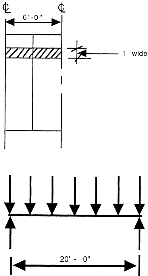
Figure 1.3 Typical beam. (a) Loading strip; (b) simply supported beam.
