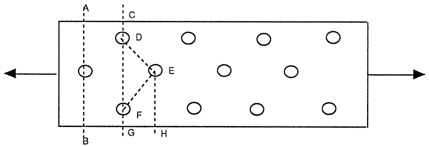
Figure 2.7 Typical staggered bolt connection.
