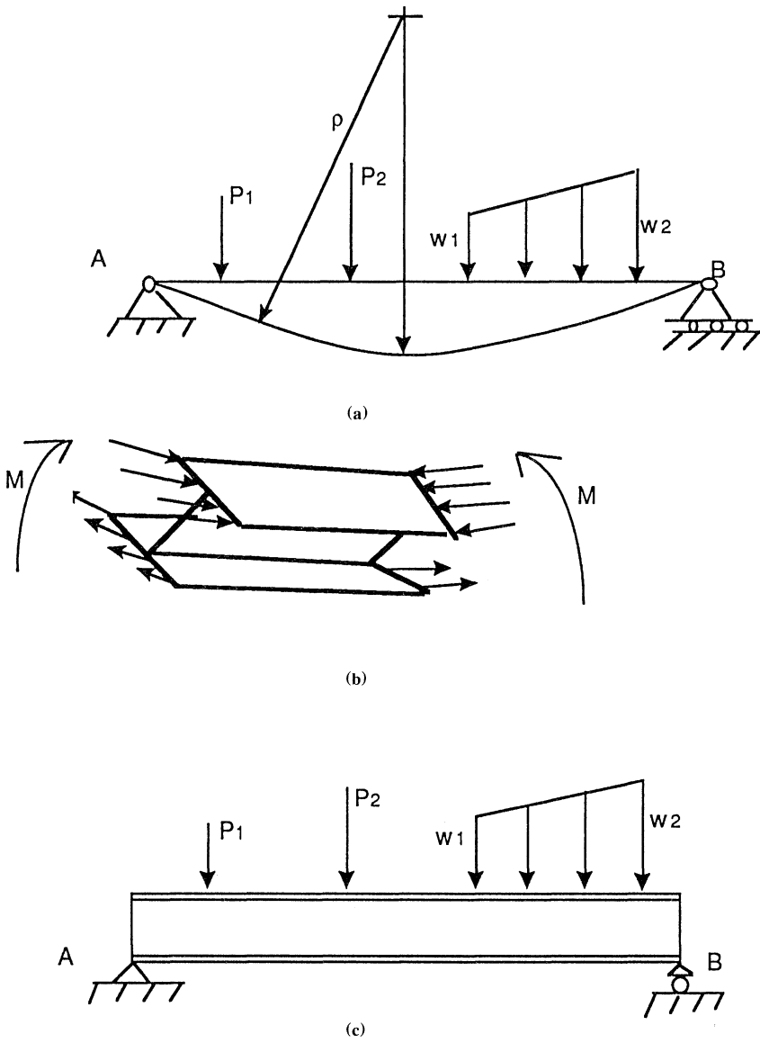
Figure 4.1 Beam deflection due to bending.
