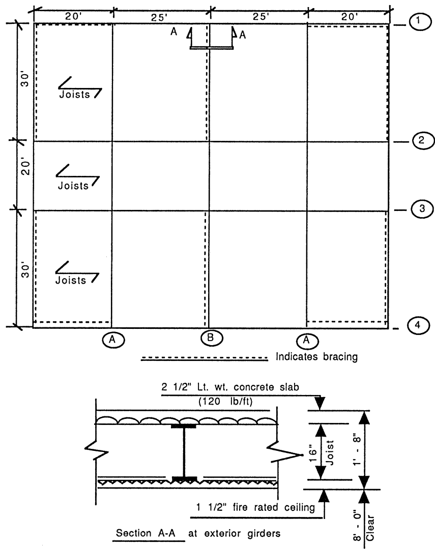
Figure 14.1 Building floorplan and section of an exterior girder.
