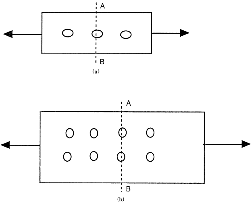
Figure 2.6 Typical connection. (a) Single row. (b) Two nonstaggered rows.
