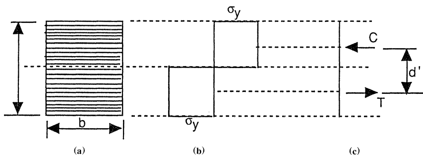
Figure 11.5 Stress distribution: Fully plastic state.
