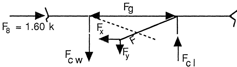
Figure 6.9 Resolution of wind shear in the braced frame.
