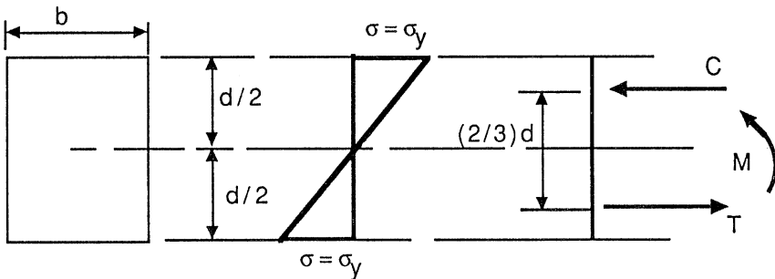
Figure 11.3 Stress distribution: Yield limit.
