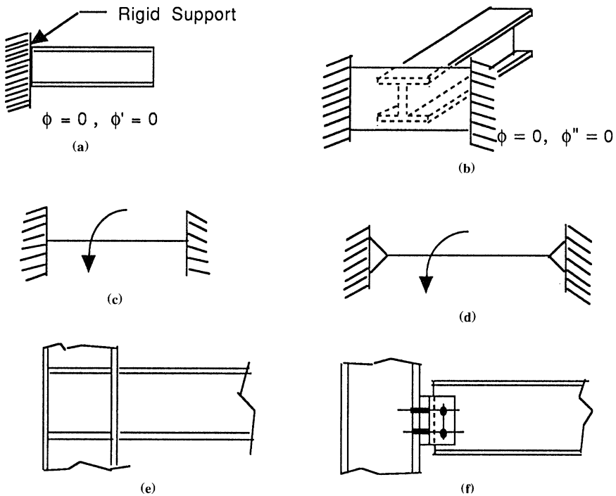
Figure 5.3 Bending stresses. (a) Ideal. (b) Ideal. (c) and (d) Schematic representations. (e) and (f) Structural connections.
