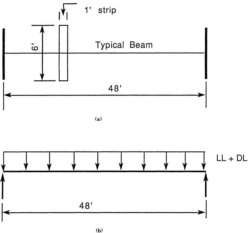
Figure 4.5 Load calculations on a typical beam.
