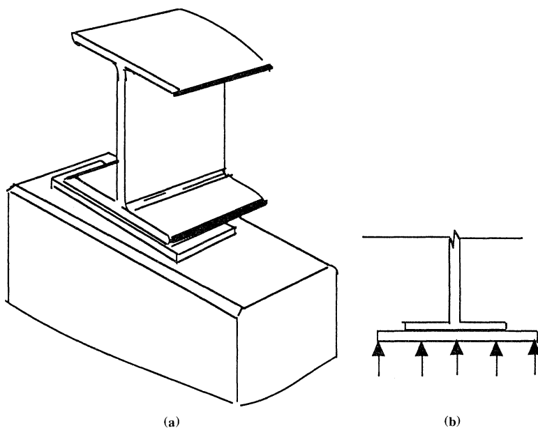
Figure 8.1 Beam baseplate.
