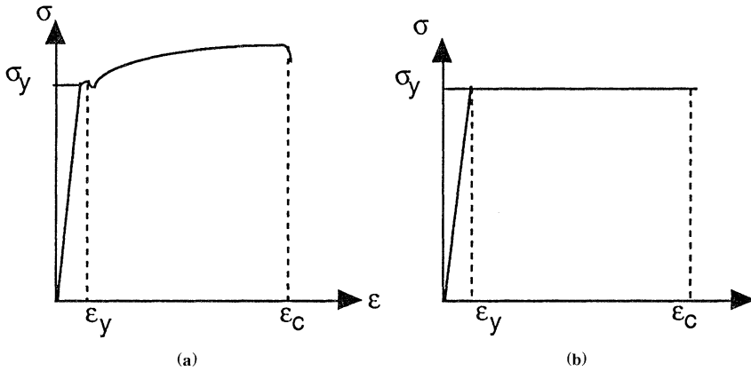
Figure 11.1 Stress vs. strain curve for structural steel. (a) Real. (b) Ideal.
