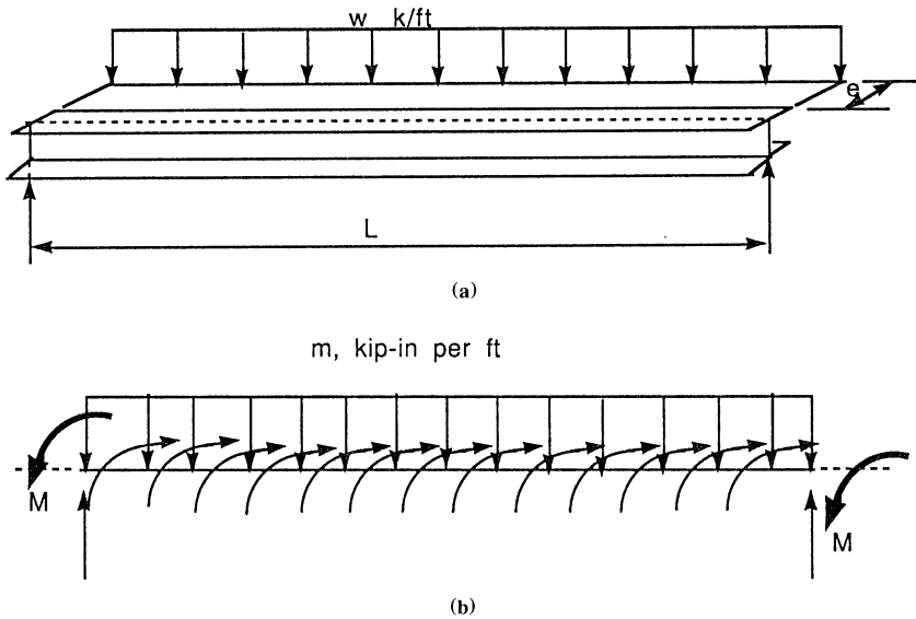
Figure 5.1 Uniform load applied outside of the plane of symmetry of a beam.
