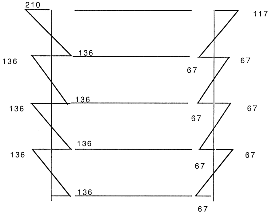
Figure 14.4 Column moment diagrams.
