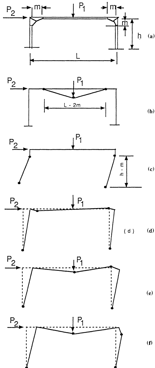
Figure 13.7 Failure mechanism for a haunched corner connection in a portal frame.
