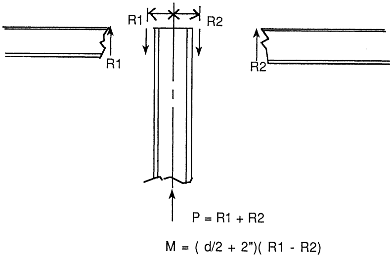
Figure 3.5 Beam/girder column reactions.
