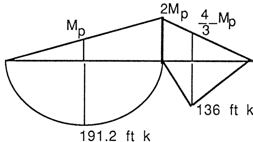
Figure 11.21 Equilibrium of moments approach.
