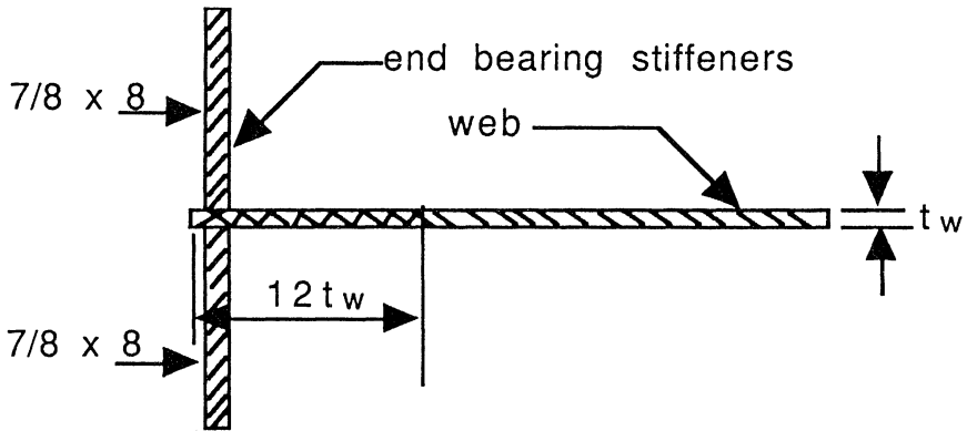
Figure 9.5 End bearing stiffener for plate girder.
