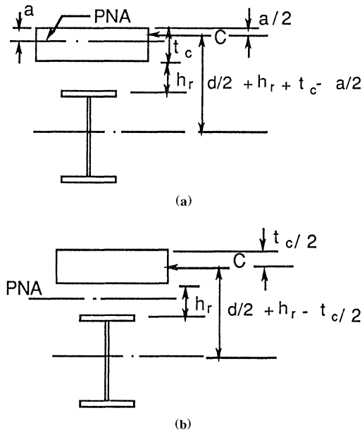
Figure 10.11 Neutral axis of composite sections using the plastic method.
