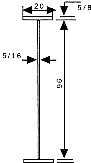
Figure 9.6 Plate girder section dimensions.
