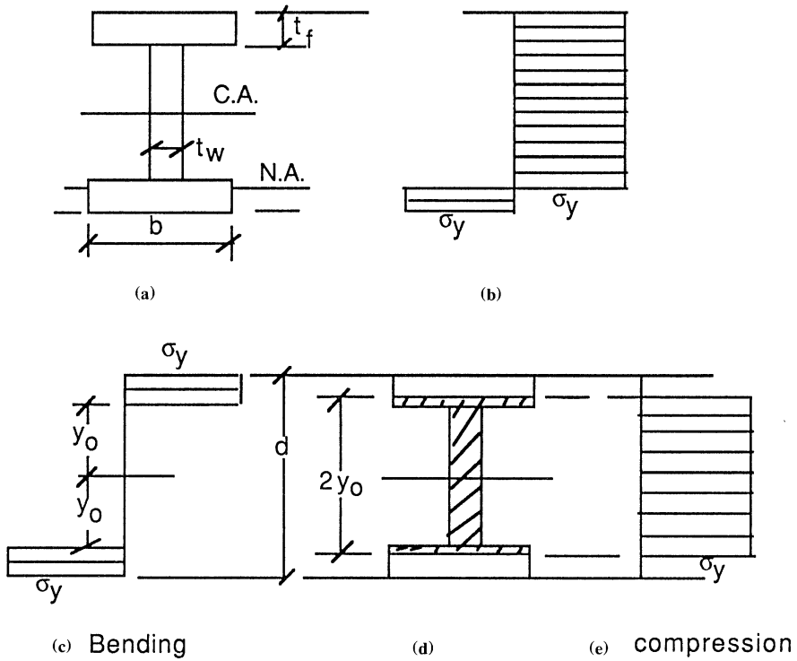
Figure 12.4 Determination of the neutral axis in the flange (a) Beam cross section. (b) Stress diagram. (c) Bending. (d) Area under compression. (e) Compression.
